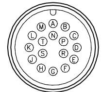
MALE END VIEW
